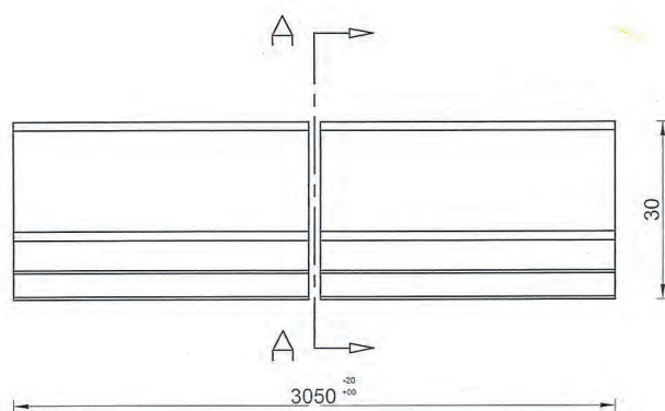
FRONTAL VIEW
